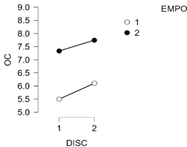
Figure 2. Descriptive Plot
